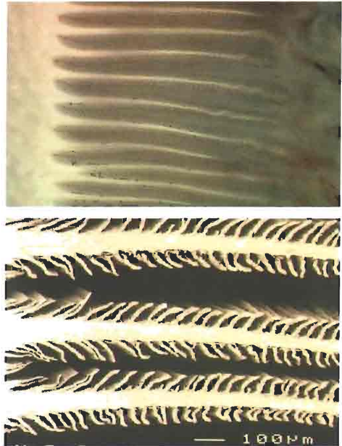
Fig 7: To increase the surface area of the inner hoof wall there are 550–600 primary epidermal lamellae (PELs). The surface area of each PEL is further increased with an extra 150–200 secondary lamellae along the length of each PEL. The tips of the lamellae (both primary and secondary) all orientate towards the distal phalanx (on the right of each picture but not shown) therefore indicating the lines of tension to which the lamellar suspensory apparatus is subjected. The upper picture is an unstained section magnified about \times 10 . The lower picture is an electron micrograph: bar 0.1 mm. In life each PEL measures about 7 mm when viewed in this plane.
